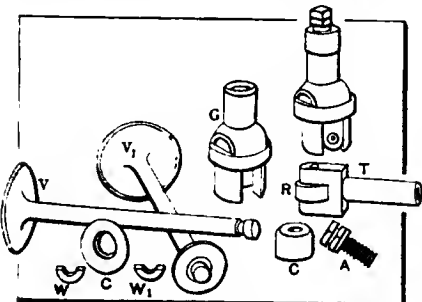
Fig. 16—Assembly of the Marmon valves and tappets
